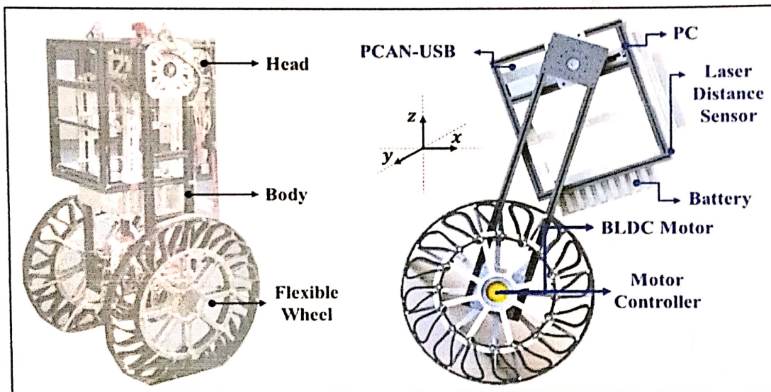
MOBINN-M3 Delivery Robot
