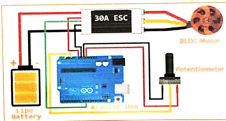
BLDC motor control circuit diagram
